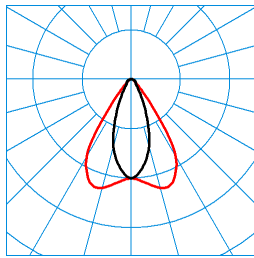
Mirona Fit HR LED70000-840 TX245374
