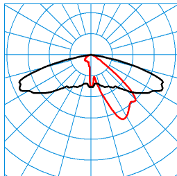
Publisca P1W-AB2L-LR/3800-740 6G1S ET (CLO initial value) TX300523 ■ C0 - C180 ■ C90 - C270 DIN 5040: A30 UTE: 1,00 G CEN Flux Code: 34 72 97 100 100 0 0 0 0
