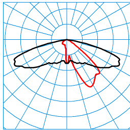
Publisca P1W-AB2L-LR/3800-740 6G1S ET (CLO end value) TX301061 ■ C0 - C180 ■ C90 - C270 DIN 5040: A30 UTE: 1,00 G CEN Flux Code: 34 72 97 100 100 0 0 0 0
