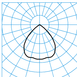
InperiaL G2 C07 BR22 1800-840 01 + RG-PC ■ C0 - C180 TX373514
