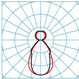
SFlow H2-L CDP-I LED6400-840 01 TX374482
