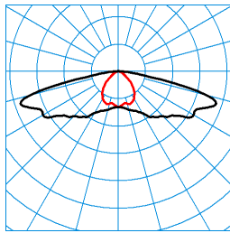
ViaCon HL-LR-SBxL5/2600-740 4G1S TX054647
