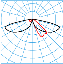
LTX L-AB2L-LRA/15/18/26-730 4G1 (1800 lm) TX061510 DIN 5040: A20 UTE: 1,00 l CEN Flux Code: 24 61 92 100 100 0 0 0 0 ■ C0 - C180 ■ C90 - C270
