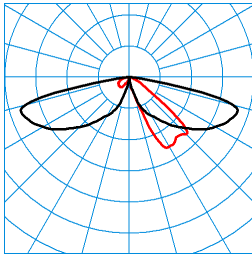
LTX L-AB2L-LRA/15/18/26-730 4G1 (1500 lm) TX076486 DIN 5040: A20 UTE: 1,00 l CEN Flux Code: 24 61 92 100 100 0 0 0 0 ■ C0 - C180 ■ C90 - C270
