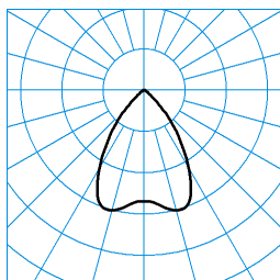
InperiaL G2 C07 BR19 1000-840 01 + RG-PC ■ C0 - C180 TX372382
