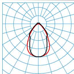
SFlow D2-L CDP-I LED4000-840 EB3 03 TX133390
