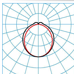
ELINE HE DL120 840 L225 1 50
