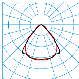
SFlow C1-L MRW LED3200-840 01 TX050941
