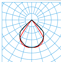
Skeo Q-W1-D GS RB9R/200-730 TX054258
