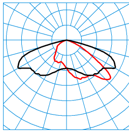
LIQ 70N-AB7L-SLR2/7500-730 8G1 ET(CLO end value) TX277771 DIN 5040: A30 UTE: 1,00 G CEN Flux Code: 35 73 98 100 100 0 0 0 0 ■ C0 - C180 ■ C90 - C270
