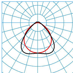
ELINE HE PW80 827-65 L225 4 50
